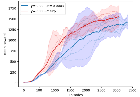
Fig. 6. Learning curves (running average on 200 episodes) for five runs of (0.99, 0.0003) in blue; and five for (0.99, exp) in red. The ticker lines are the mean over the five curves, while the semi-transparent are the 2 \cdot \sigma (standard deviation), representing the 95% probability of finding other curves in that space. Generally the pair (0.99, exp) performed better.
